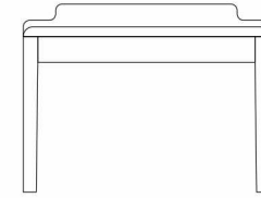
LUGGAGE BENCH 30W X 20D X 19H ARLB
