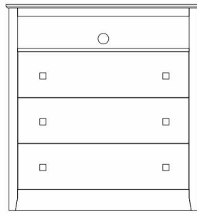
3 DRAWER CHEST 36 1/4W X 22D X 38 1/4H AR3DR
